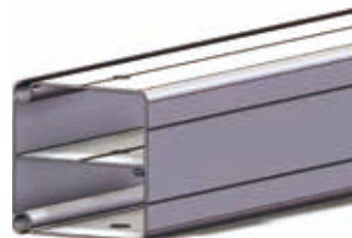
名称：前后横梁 材质：铝合金 规格：80*80*1.4mm Name: Front and rear crossbeam Material: Aluminum alloy Specifications: 80*80*1.4mm
