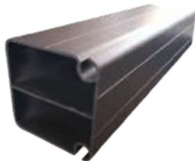
名称：前后横梁 材质：铝合金 规格：60*60*1.4mm Name: Front and rear crossbeam Material: Aluminum alloy Specifications: 60*60*1.4mm
