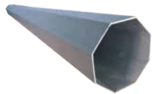
名称：八角传动管 材质：铝合金 规格：直径70*70*1.3mm Name: Octagonal drive tube Material: Aluminum alloy Specifications: Diameter 70*70*1.3mm
