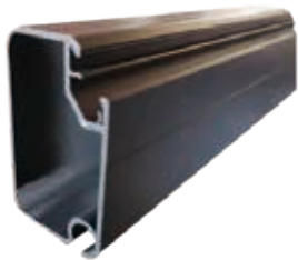
名称：中横梁 材质：铝合金 规格：60*36*1.4mm Name: Middle crossbeam Material: Aluminum alloy Specifications: 60*36*1.4mm
